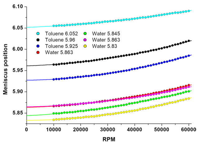
Fig. 5 Representative meniscus positions measured from the forward-speed experiments with toluene and water samples as a function of speed from 10,000–60,000 rpm (filled circles). The numbers in the legend indicate the meniscus positions observed at 3000 rpm, and a second-order polynomial fit is shown for each data set that is extrapolated to the predicted meniscus position at zero rpm (solid lines). A slight increase in the curvature is apparent with increasing column length due to the increase in pressure (also see Figs. 1, 2)
